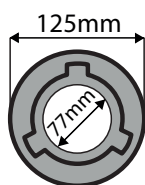
Triple bayonet with Internal flange
