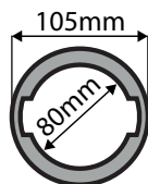
Double bayonet
